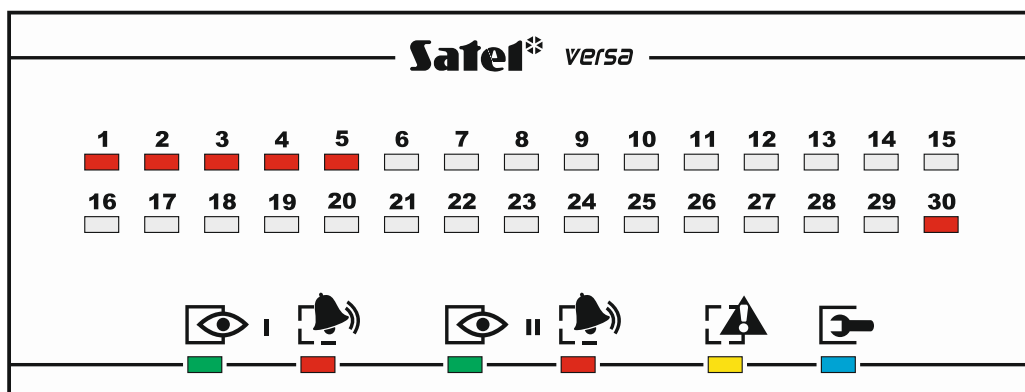
Fig. 27. Programming LED keypad address. LEDs designated with numbers from 1 to 5 and 30 are used for address presentation (30 – for address 0). The LED corresponding to the current address is flashing rapidly, the other ones are lit.
