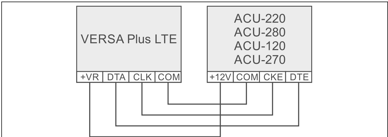
Fig. 7. Connecting the ACU-220 / ACU-280 / ACU-120 / ACU-270 controller to the control panel.
