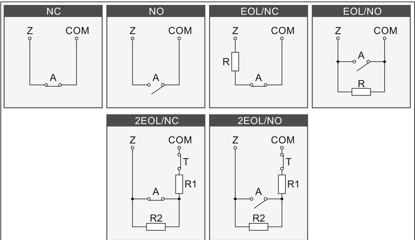
Fig. 16. The ways to connect detectors to zones. The detector outputs are designated with letters: A - alarm, T – tamper. R=R1+R2 .
