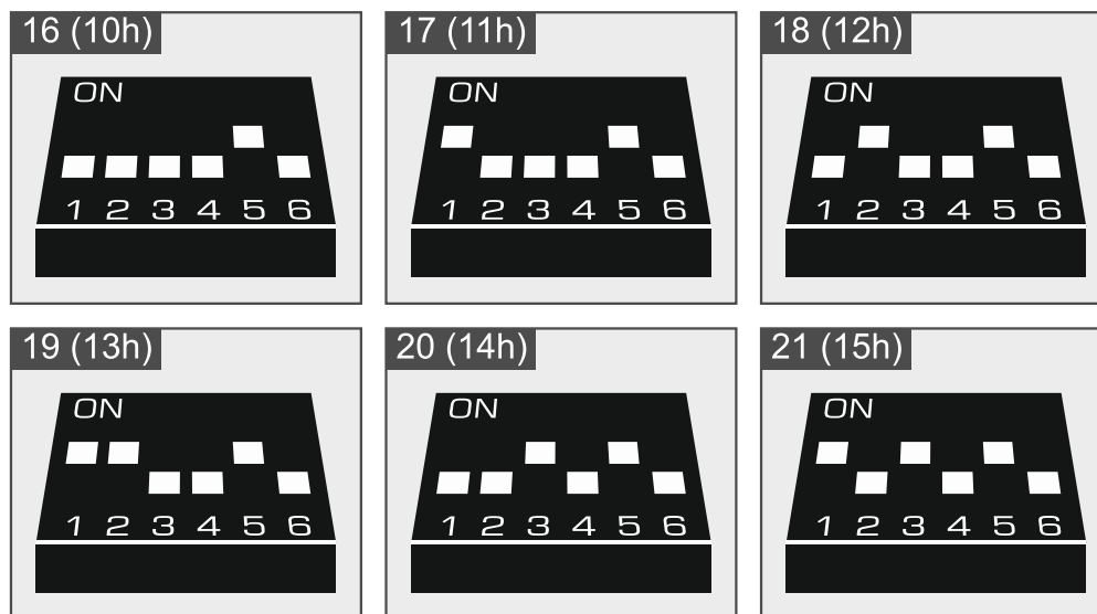
Fig. 15. Setting the address, as in the case of the INT-IT / INT-IT-2 module.
