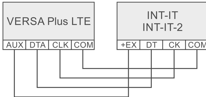
Fig. 14. Connecting the INT-IT / INT-IT-2 module to the control panel.
