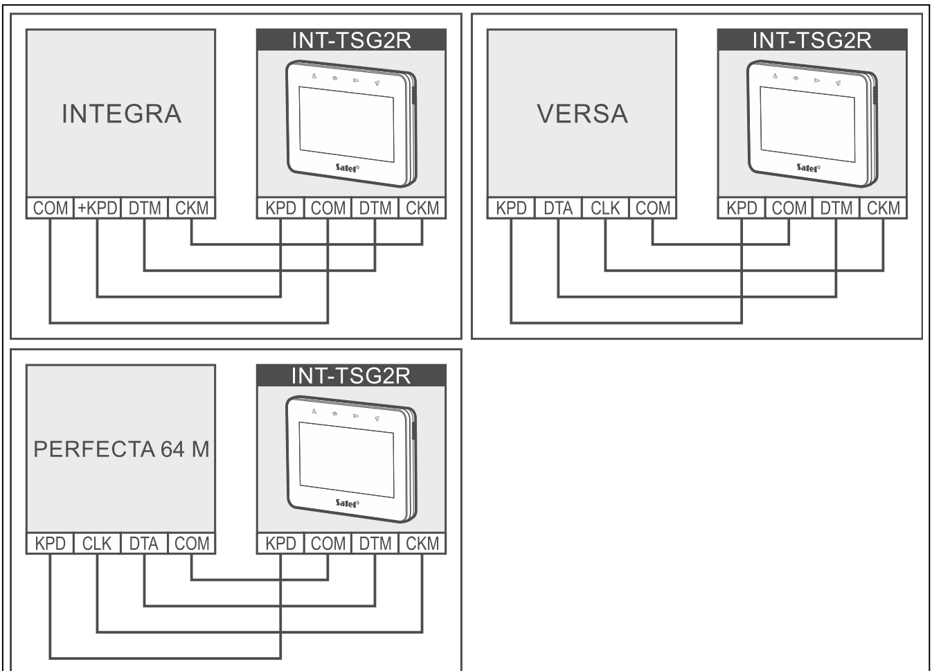
Fig. 2. Connection of the keypad to the control panel.
