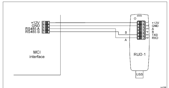
Fig. 2 Connection of the MCI-3 to RUD-1 interface for firmware update
