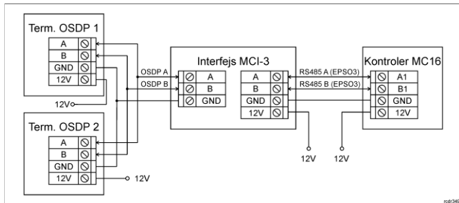
Fig. 5 Connection of MCI-3 interface to OSDP readers and MC16 controller
