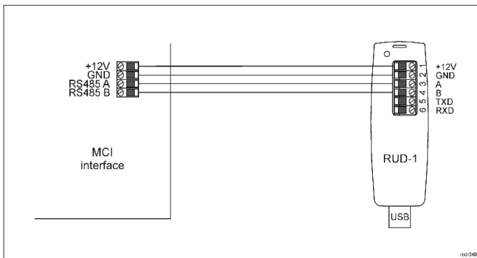
Fig. 1 Connection of the MCI-3 to RUD-1 interface for configuration
